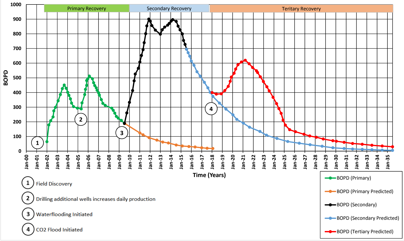
Production Decline Curve Illustrating Primary, Secondary and Tertiary Phases of Production for an Oil field.
